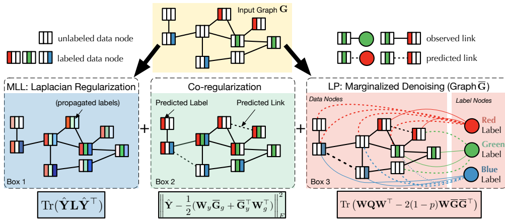
Figure 1: An illustration of MLLP. Each data node can be associated with one or more labels in a label set: Red, Green, and Blue. The original graph is augmented into a bi-relational graph, \bar{\mathbf{G}} (Box 3). The joint model (Box 2) encourages agreement between the predicted labels from MLL (Box 1) and the enriched labels from LP (Box 3).
