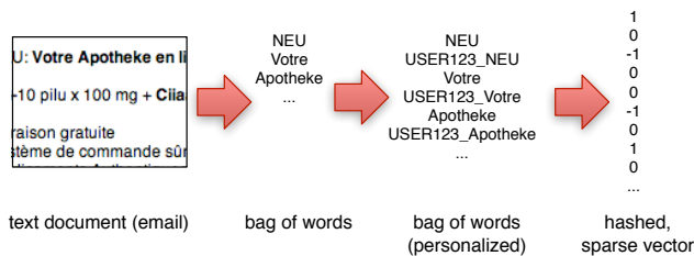
Figure 1. The hashed personalization summarized in a schematic layout. Each token is duplicated and one copy is individualized (e.g. by concatenating each word with a unique user identifier). Then, the global hash function maps all tokens into a low dimensional feature space where the document is classified.
