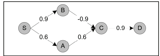
Figure 3. Revisiting the problem of negative trust.
