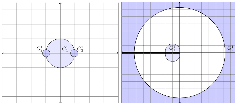
FIG. 3.1. Gershgorin regions in Example 2 (left) and Example 3 (right). In Example 2, the second Gershgorin region consists of two pieces, and the union of G_1^1 and G_2^1 contains three eigenvalues. In Example 3, neither Gershgorin region contains eigenvalues; but both \bar{G}_1^1 and \bar{G}_2^1 intersect (-\infty, 0] , which is not in the domain \Omega for this problem.
