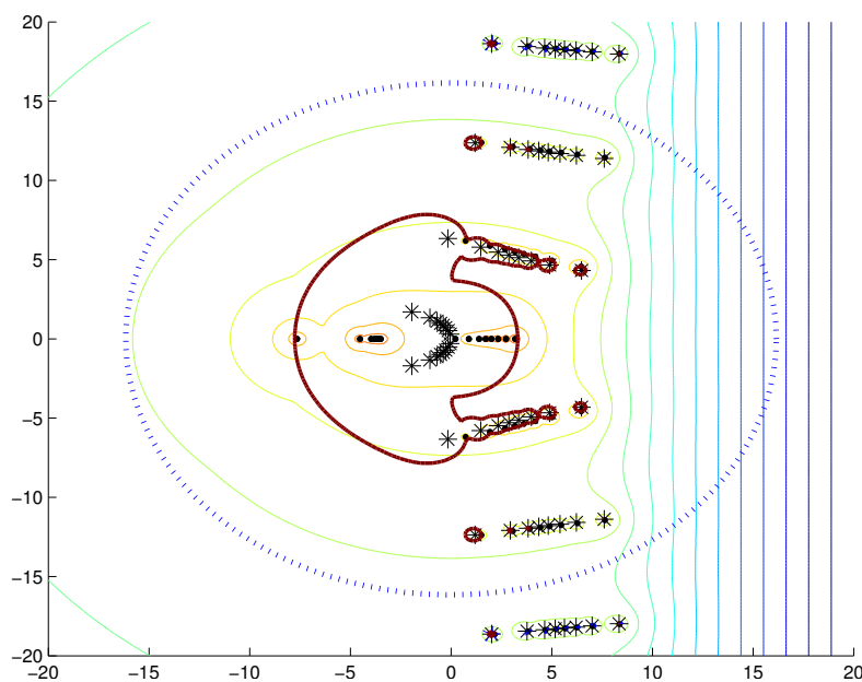
FIG. 6.5. Geršgorin region (solid line) containing eigenvalues of the Hader function T (dots) and the simplified problem \hat{T} (stars). Each connected component contains the same number of eigenvalues for both problems. The Geršgorin region is somewhat complicated, but it can be shown that the components of the Geršgorin regions containing eigenvalues \hat{\lambda} \in \Lambda(\hat{T}) outside a disk of radius about 16.3 (dashed line) is contained in a union of disks of radius O(|\hat{\lambda}|^{-2}) .
