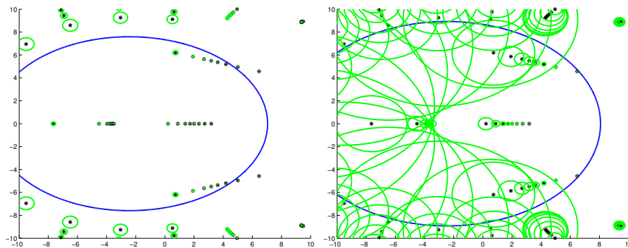
FIG. 6.4. Region where the interpolation error r(z) for the Chebyshev approximation to \exp(z) - 1 is bounded by \epsilon = 0.1 (left) and \epsilon = 1.6 (right). The Geršgorin disks of radii \epsilon\rho_j are shown in green in each case.
