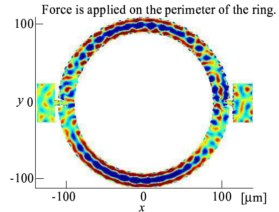
Fig. 4. Geometry, deformed shape, and thermal fluctuations of the Ring resonator at 705.50[MHz]
