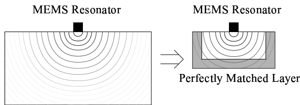
Fig. 2. Perfectly Matched Layers for Anchor Loss Simulations
