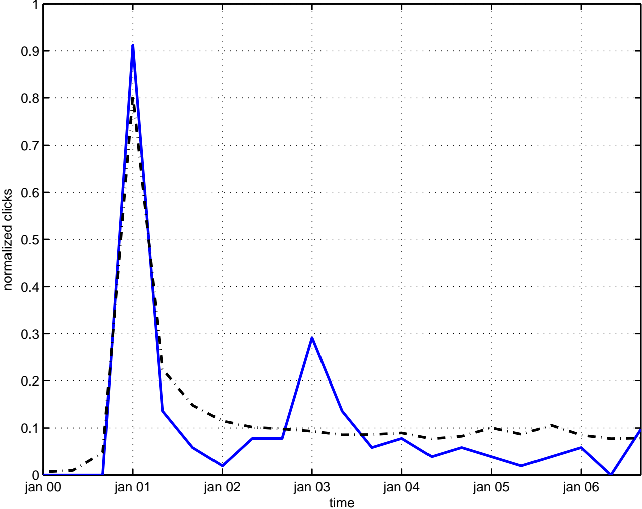
zero mode neutrino
