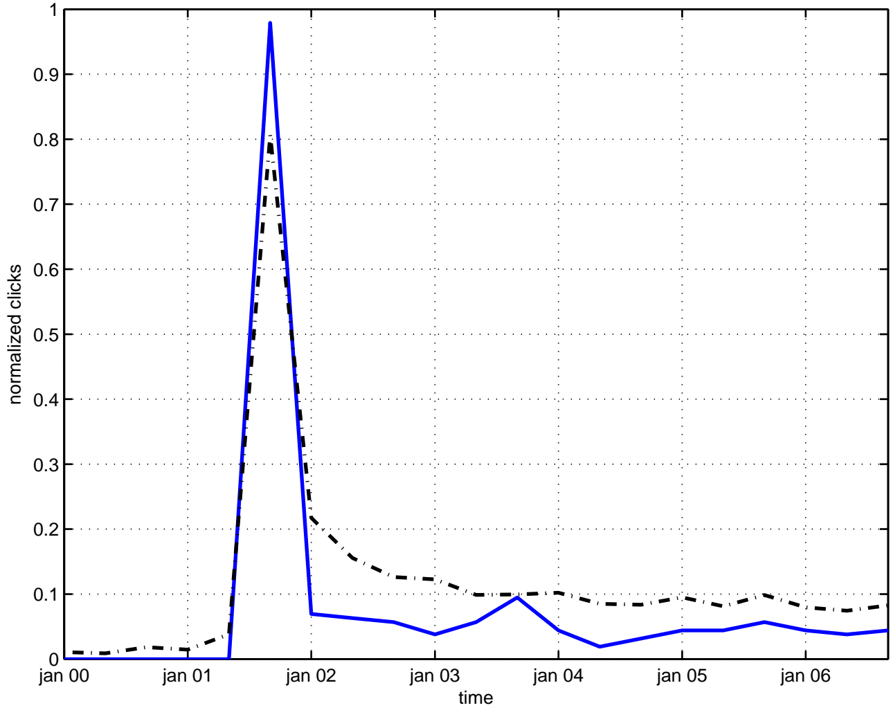
z(n)^{**m} symmetry
