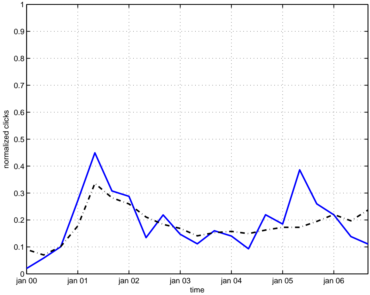
z(n) symmetry
