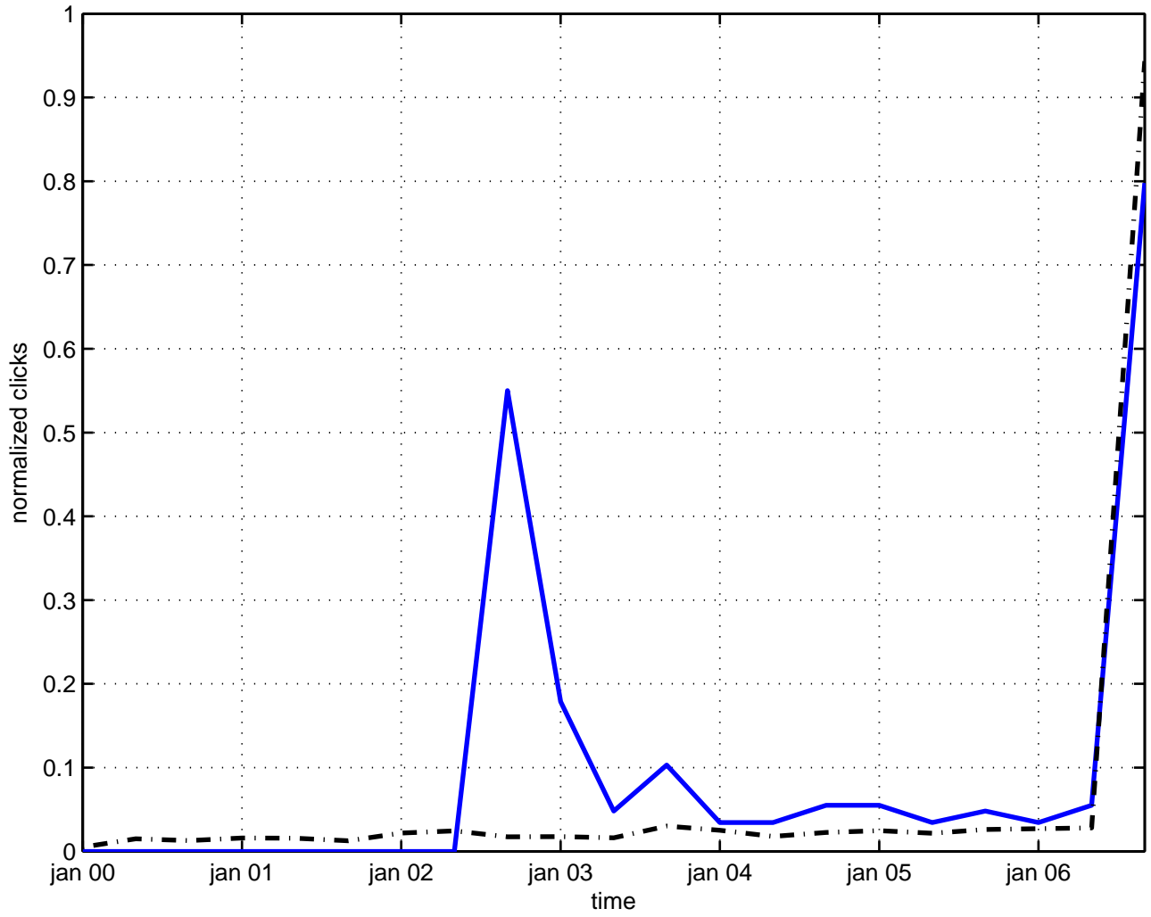
z(5) symmetry
