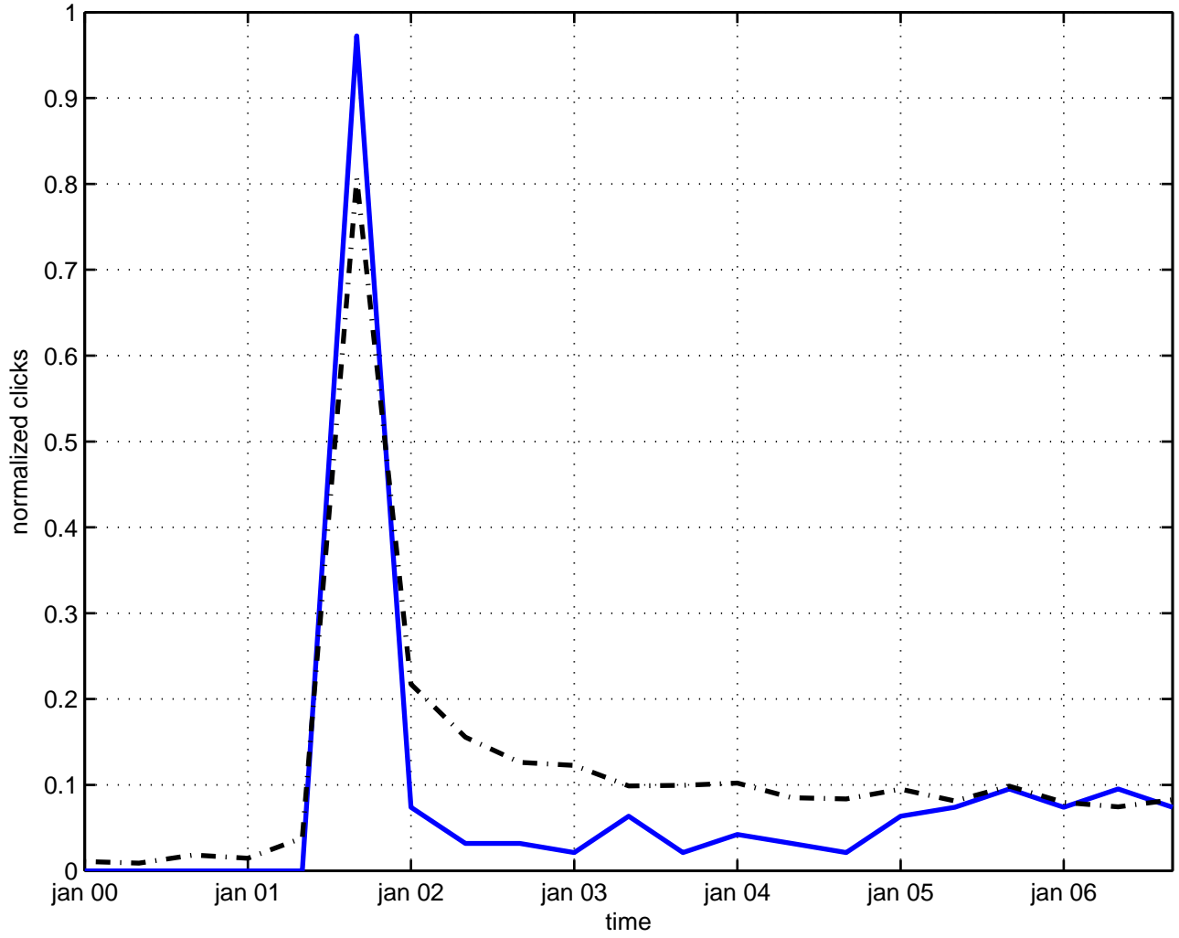
z(4)/t(2) orbifold
