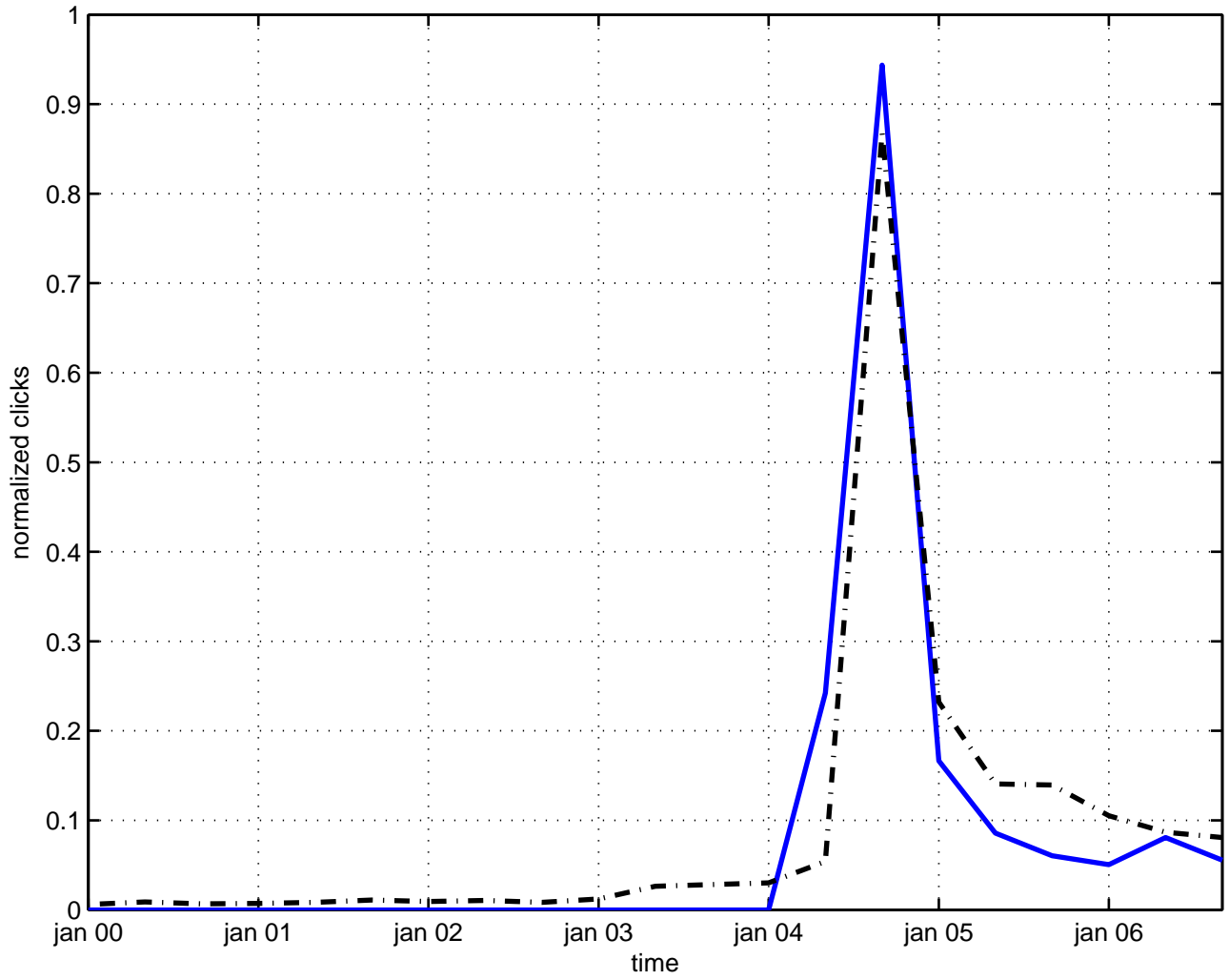
z(3) sigma model
