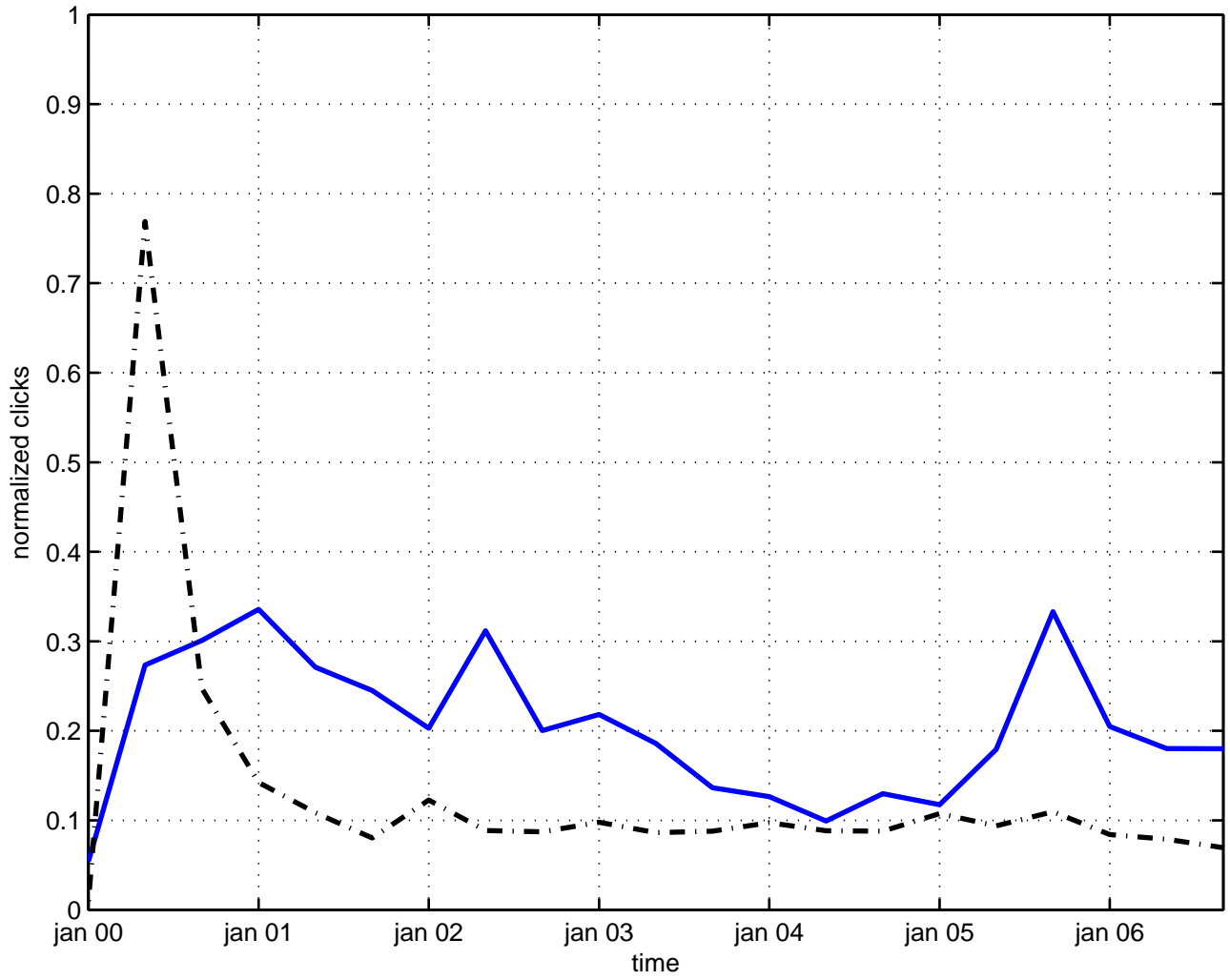
z(2) symmetry
