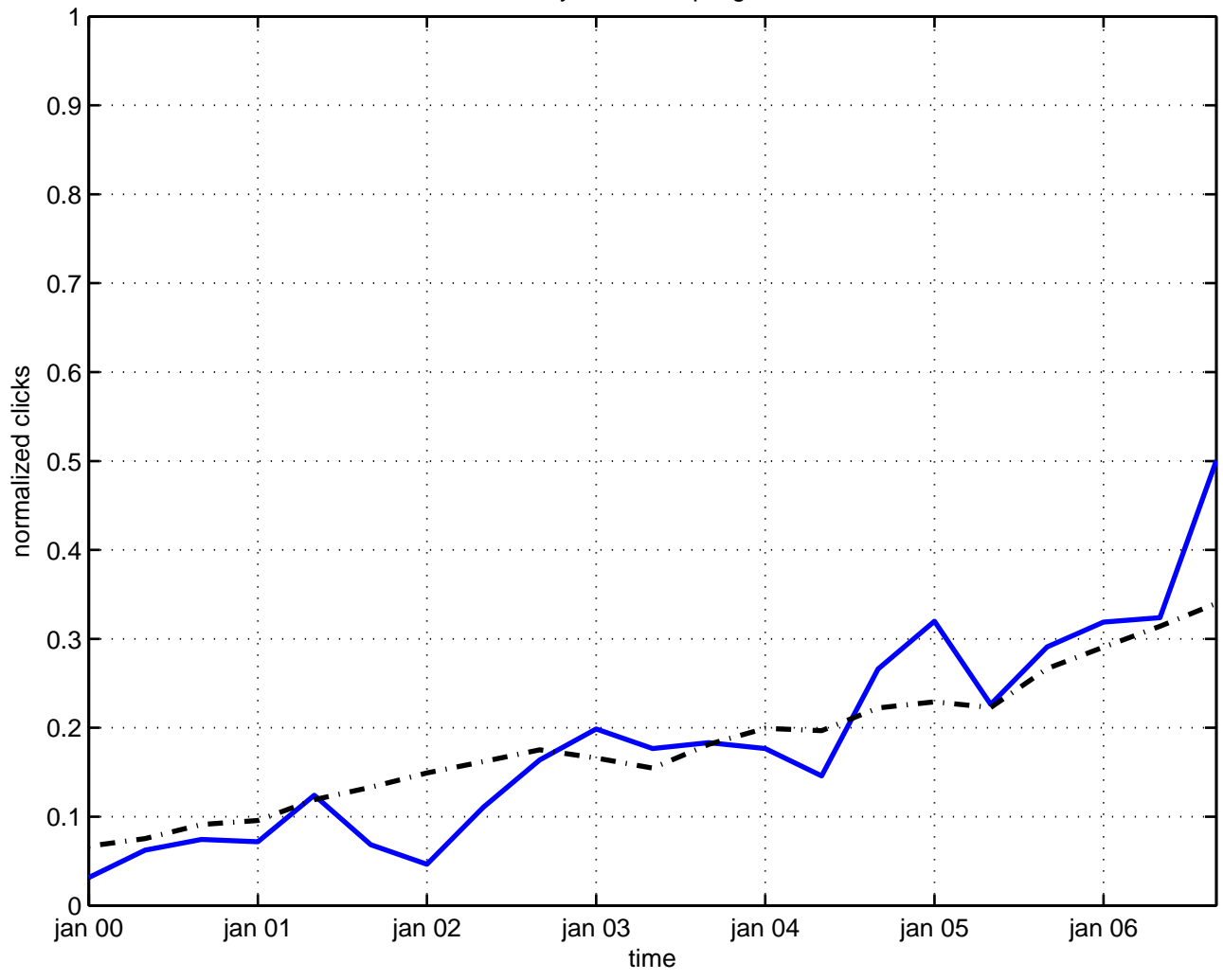
yukawa coupling
