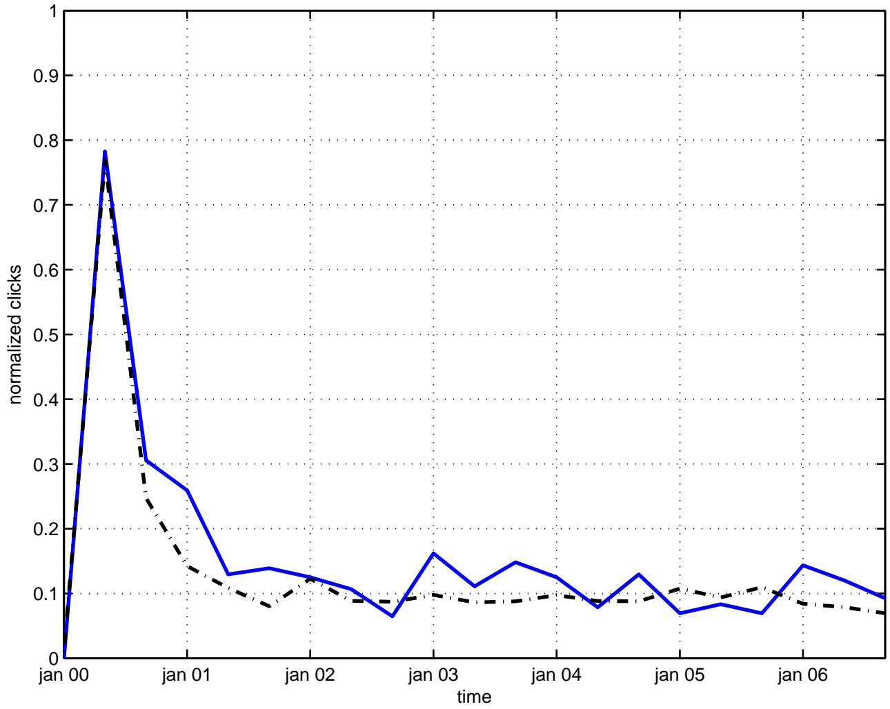
yang-mills
