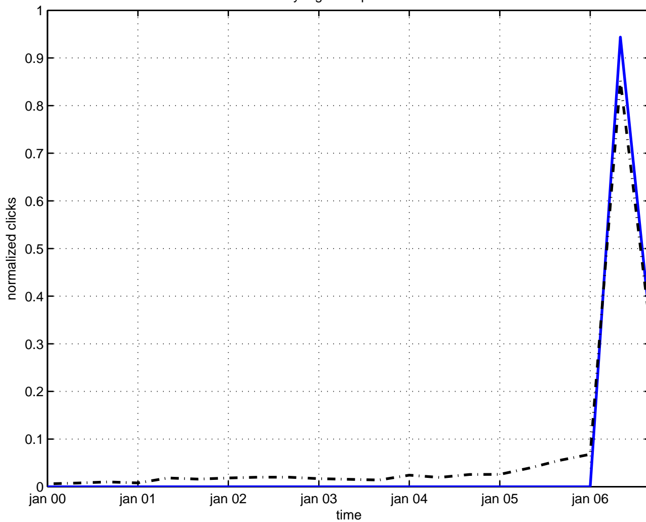
yang-mills plasma
