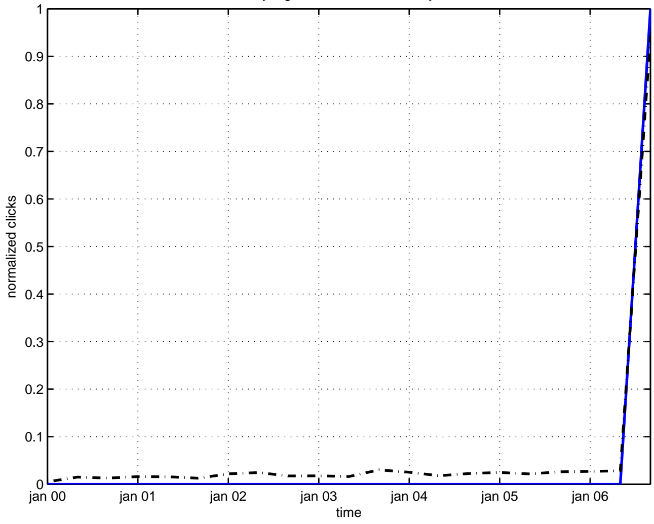
yang-mills lattice field theory
