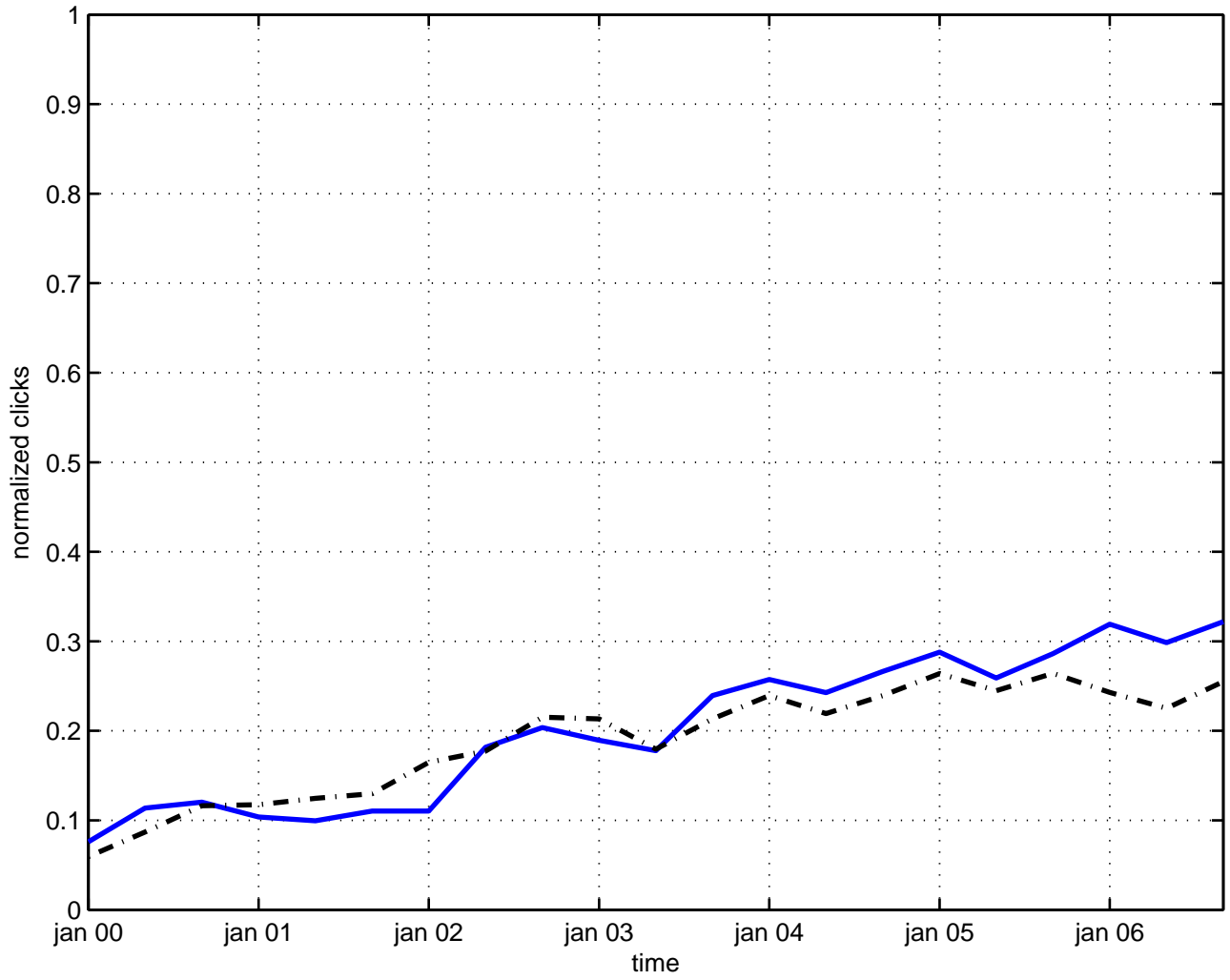
yang-mills gauge field theory
