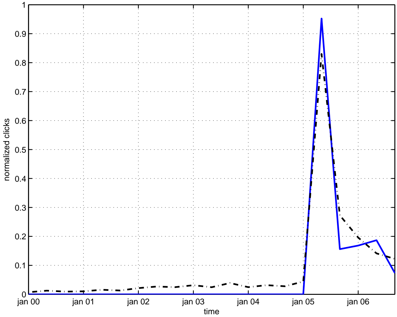
yang-mills gas
