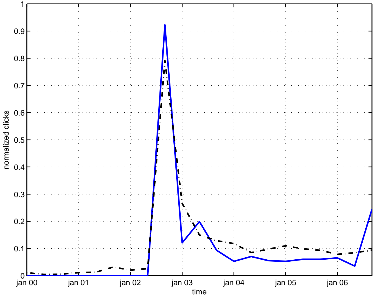
yang-mills field equations
