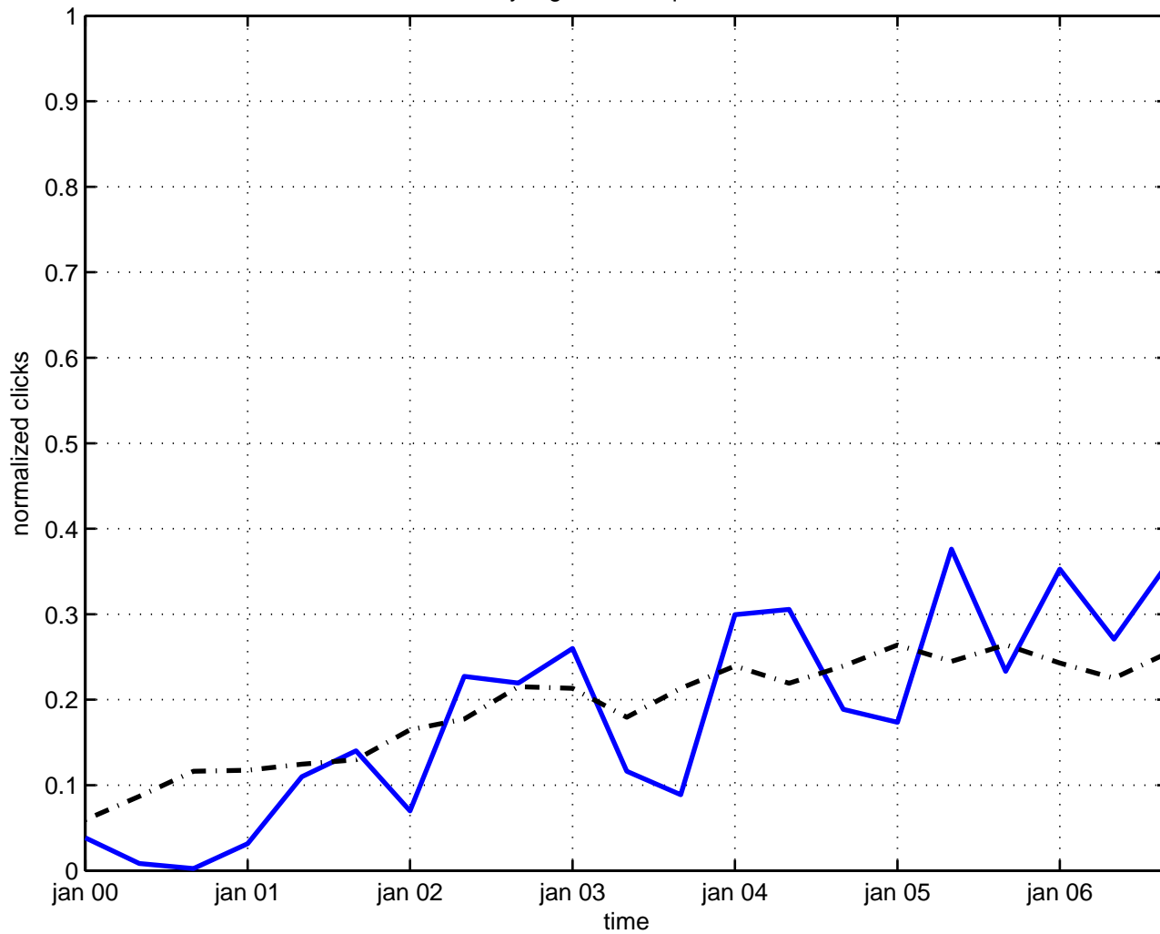
yang-baxter equation
