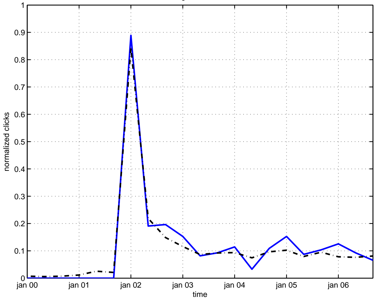
wigner function
