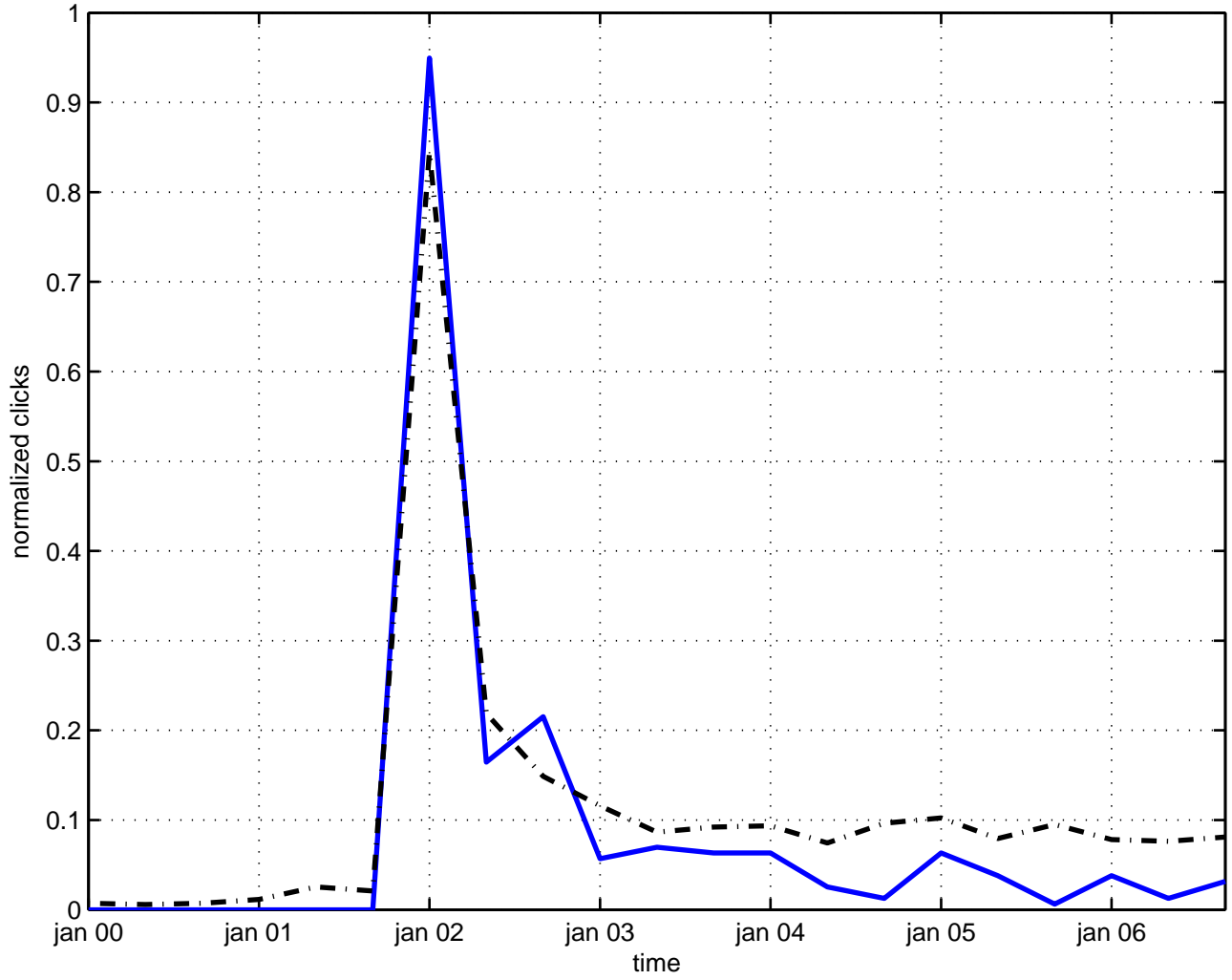
width higgs particle
