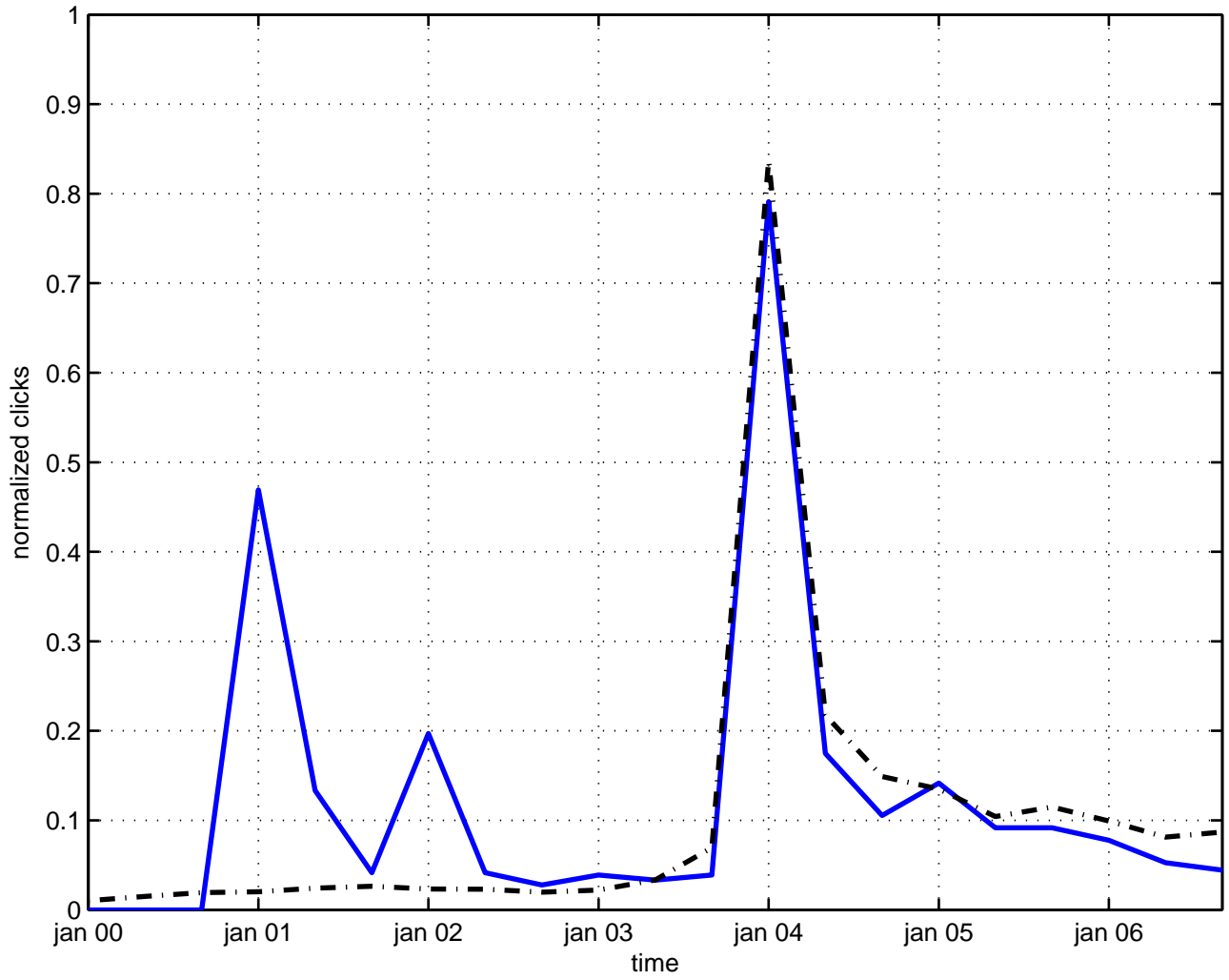
width graviton
