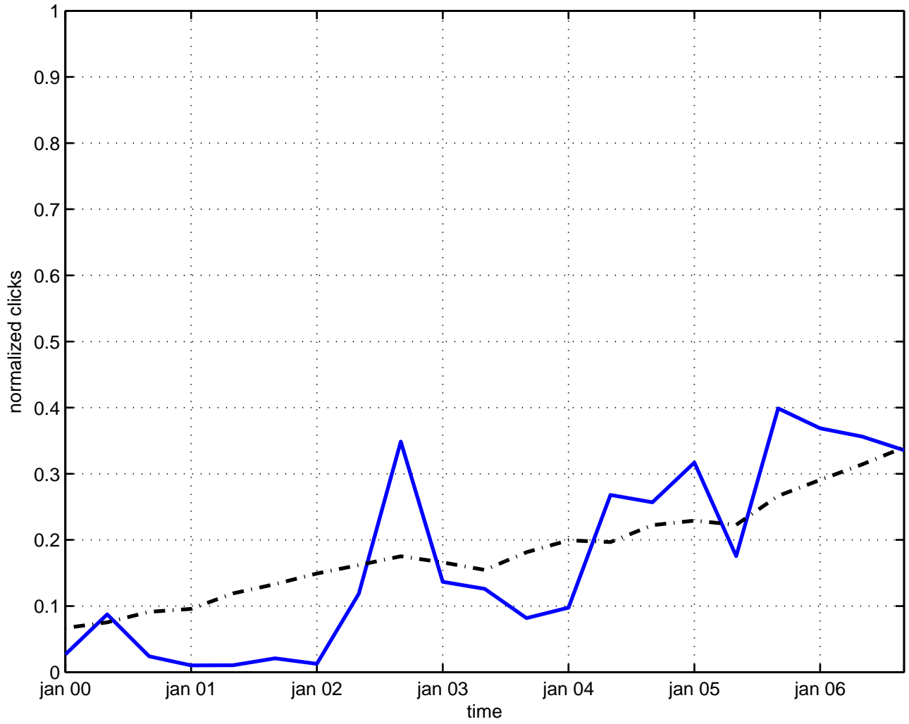
wheeler-dewitt equation
