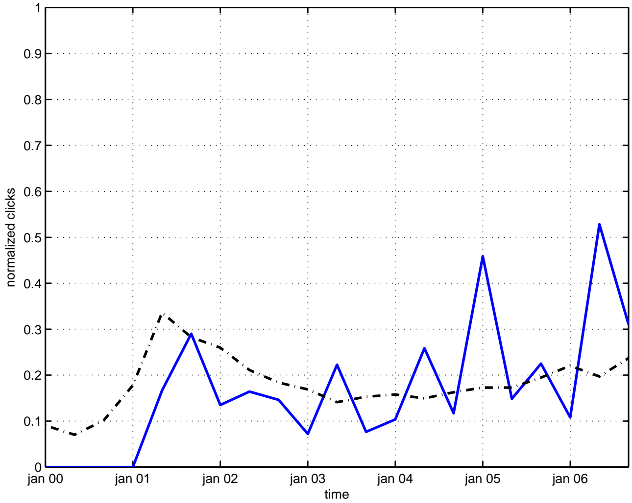
weyl symmetry
