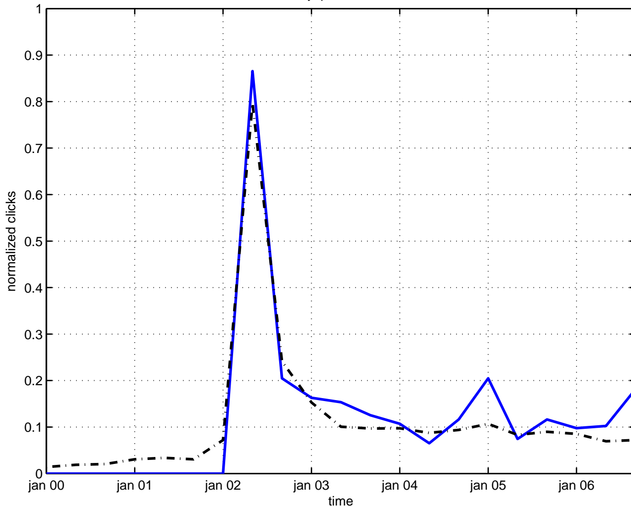
weyl perturbation
