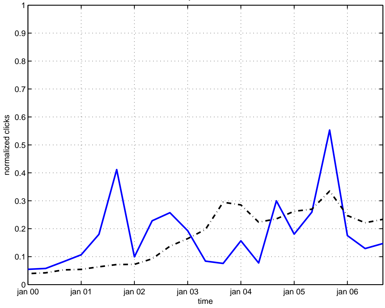
weyl invariance
