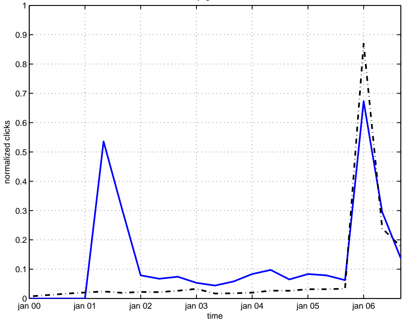
weyl gravitation
