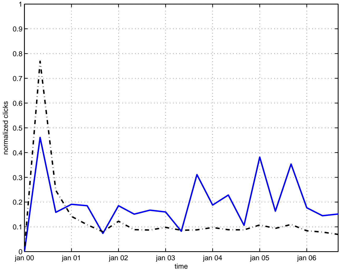
weyl anomaly
