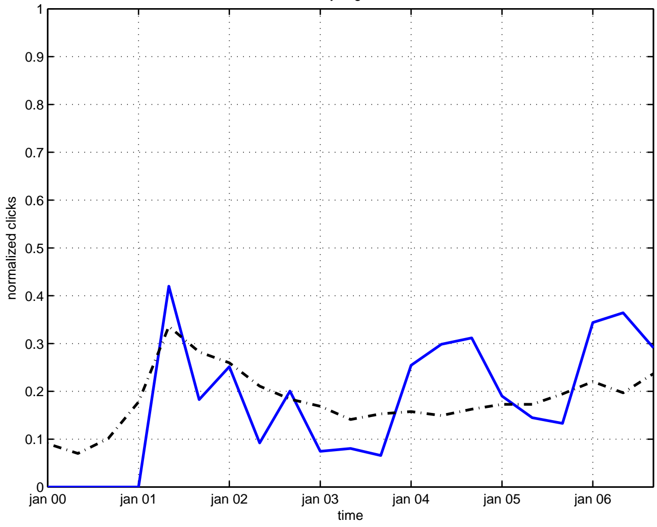
weyl algebra
