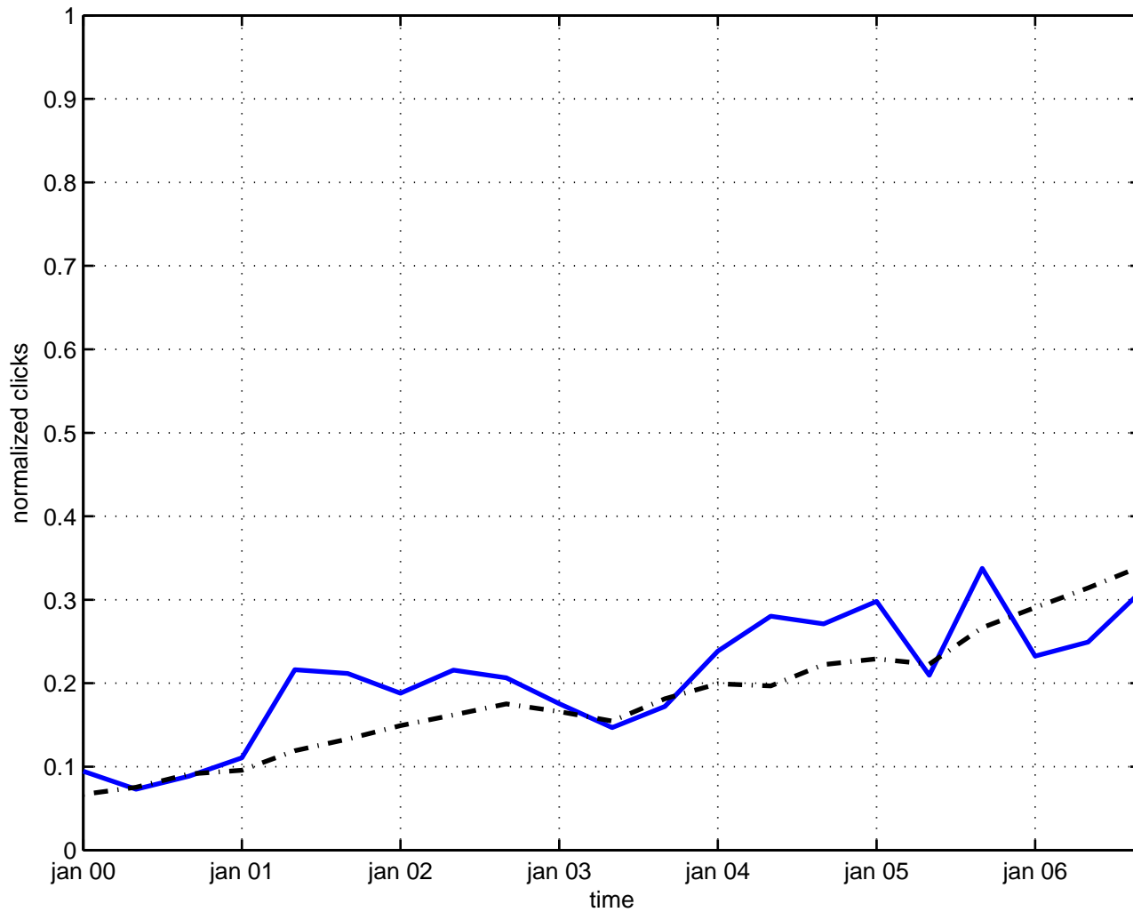
wess-zumino-witten model
