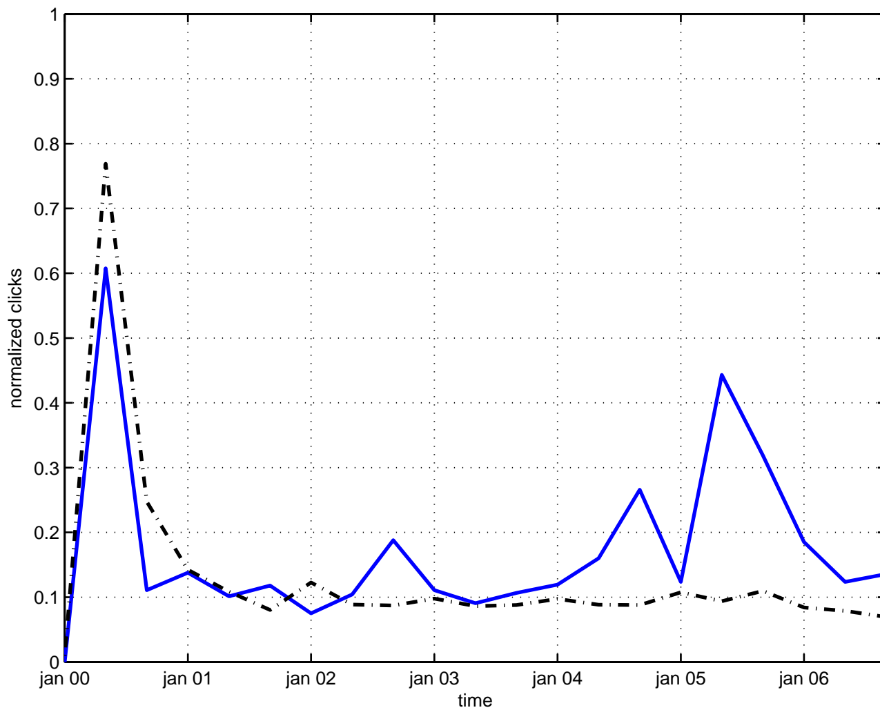
weak interaction
