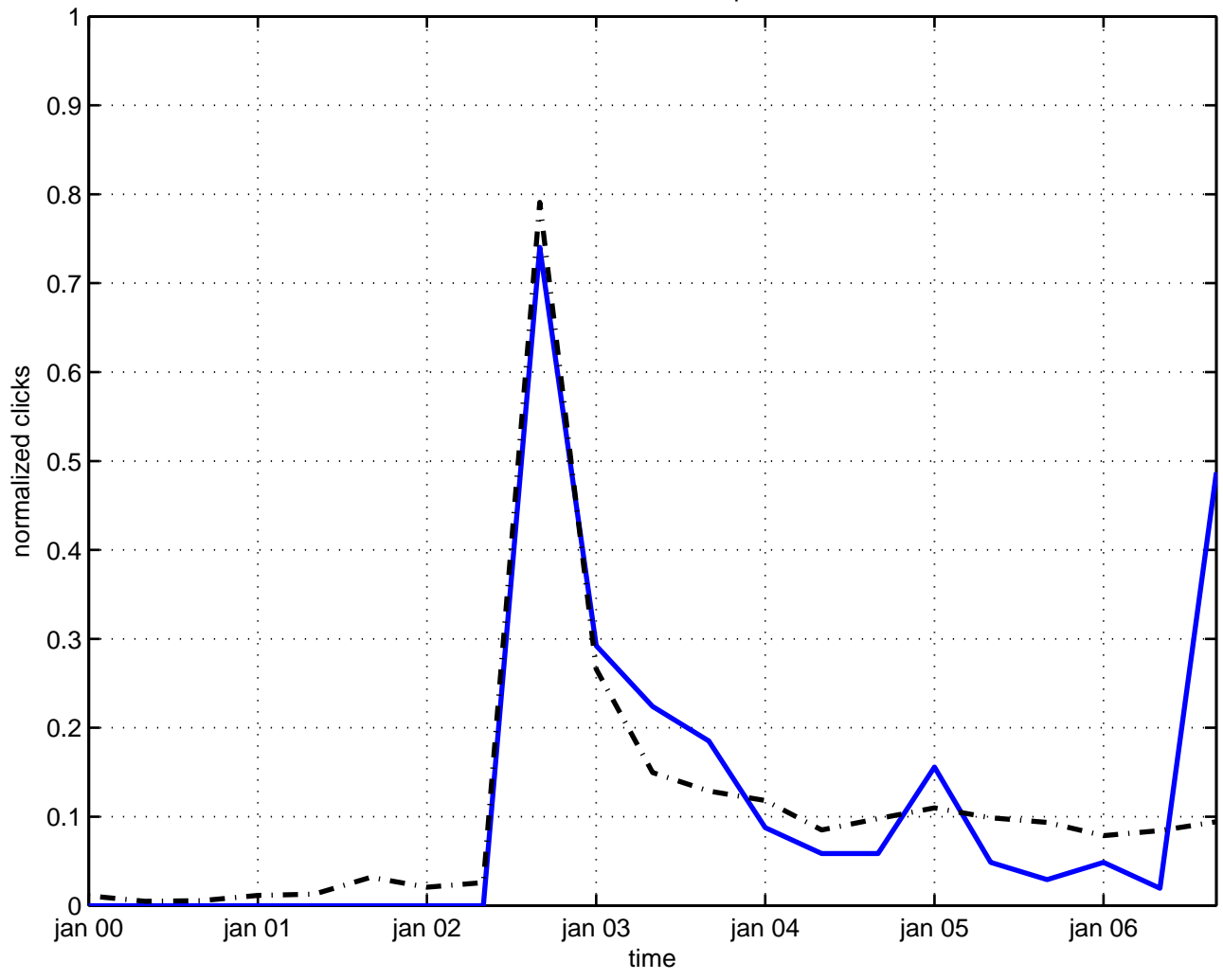
weak interaction pi
