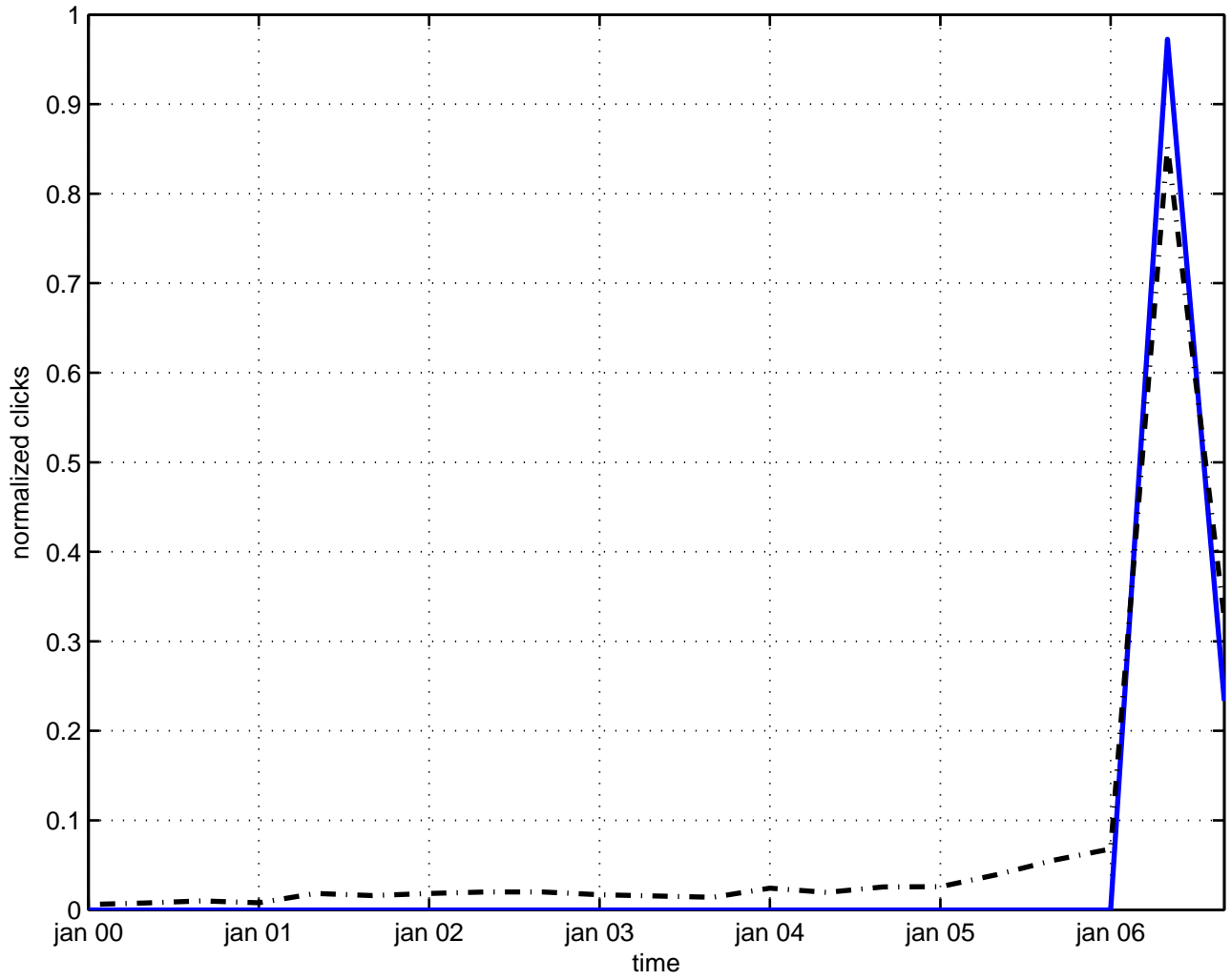
weak coupling d-brane
