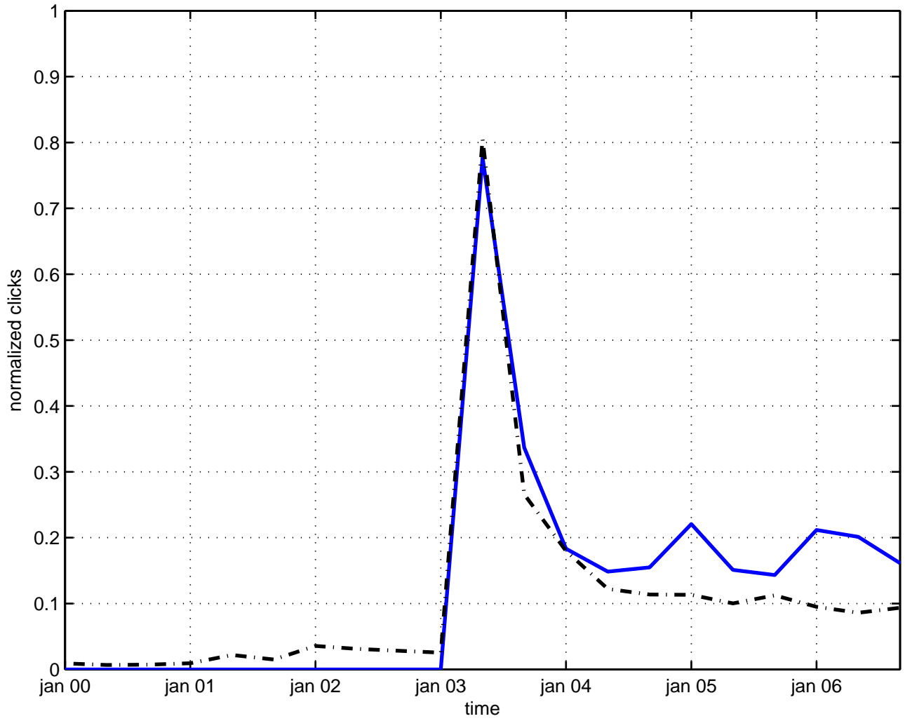
wave function quantum gravity
