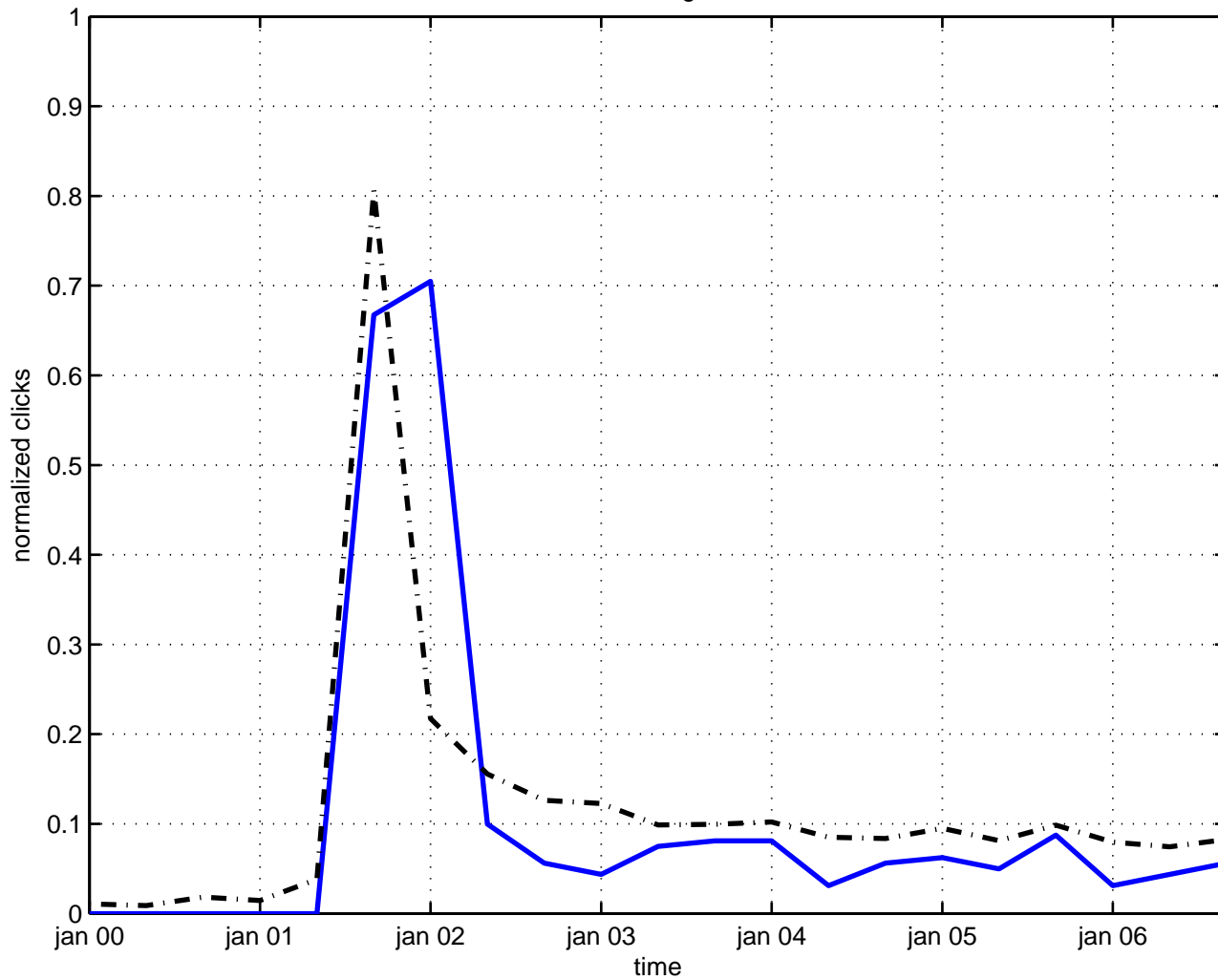
wave function gravitation
