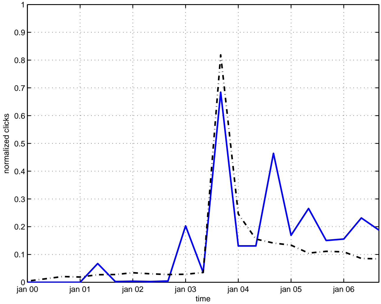
wave function astrophysics
