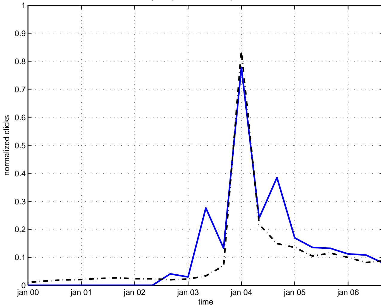
warped spontaneous compactification
