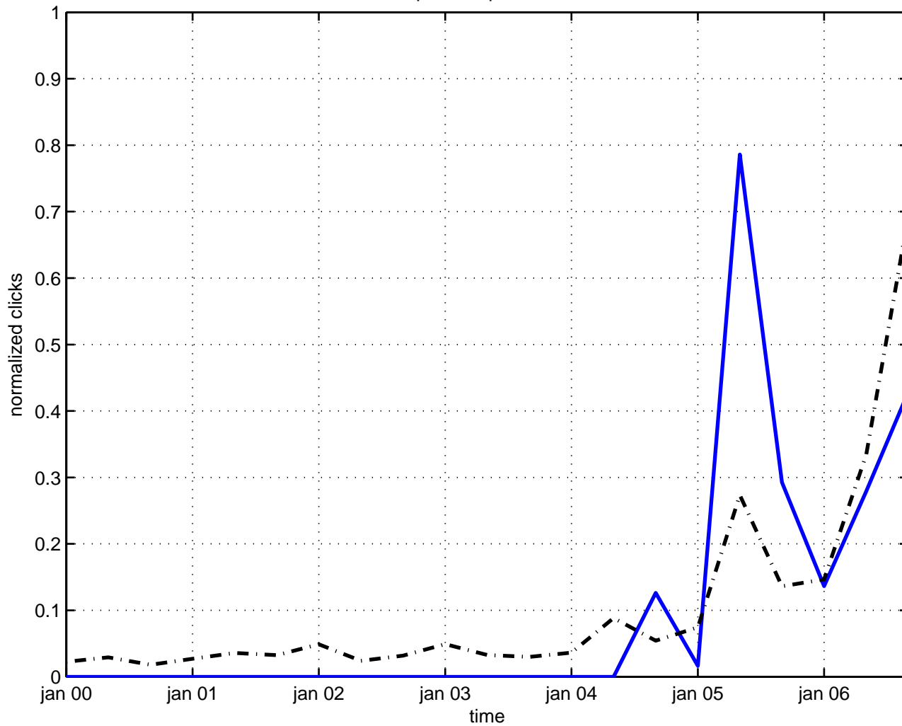
warped compactification
