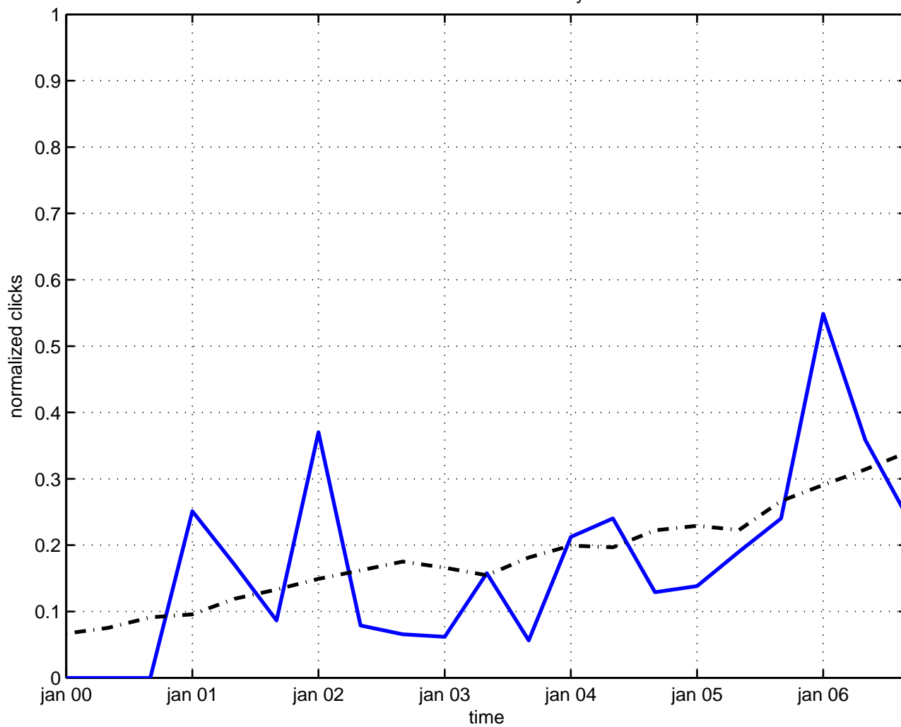
ward-takahashi identity
