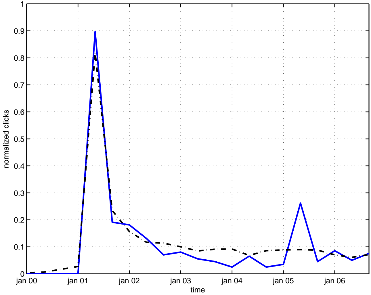
w(n) string model
