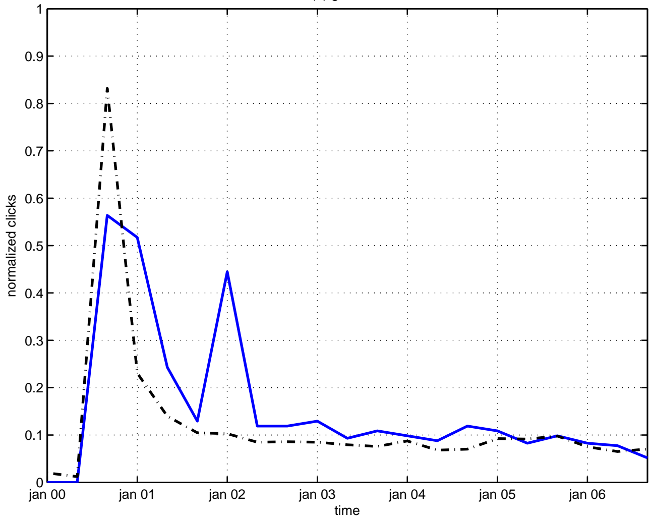
w(n) gravitation
