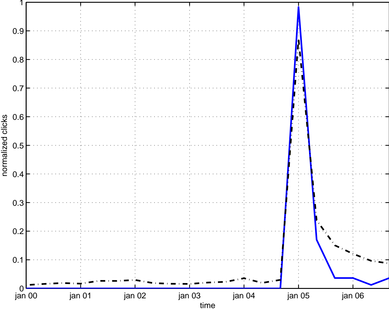
w(infinity) charge
