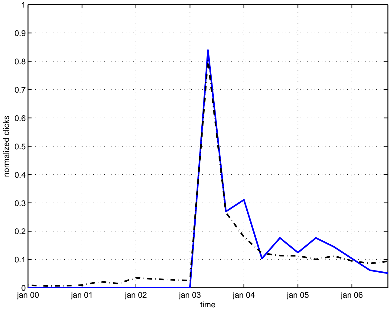
w(3) symmetry
