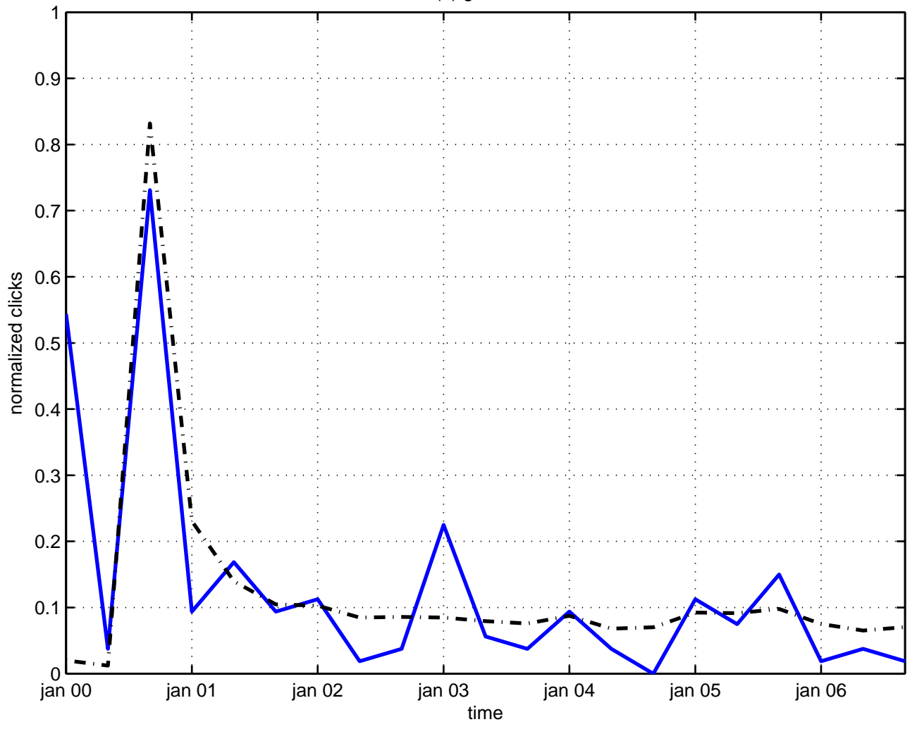
w(2) gravitation
