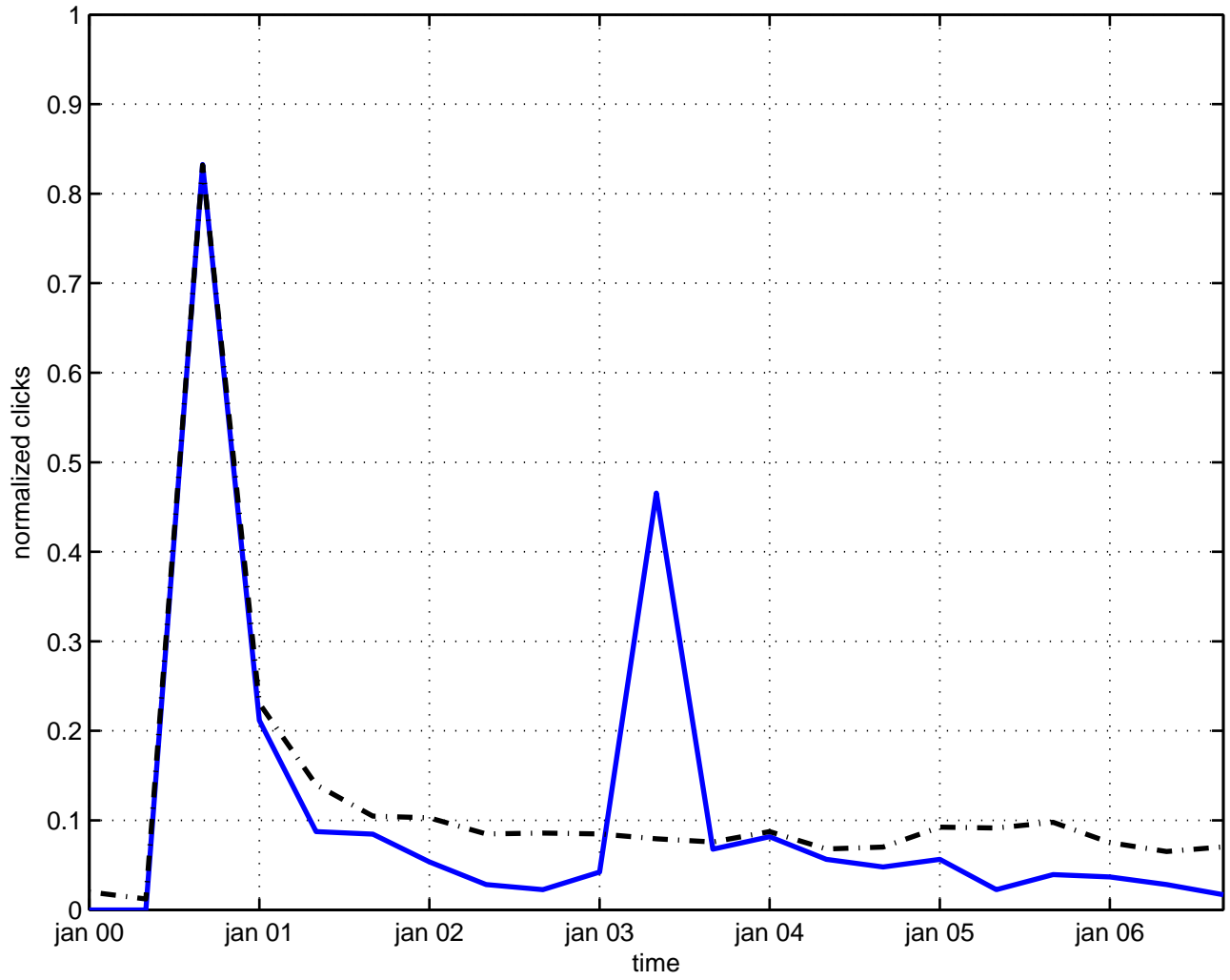
vortex field theory
