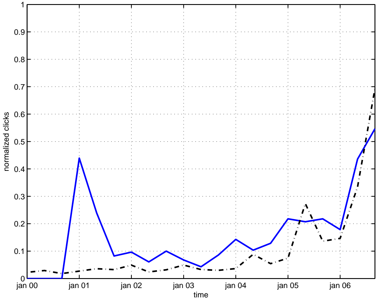
viscosity plasma
