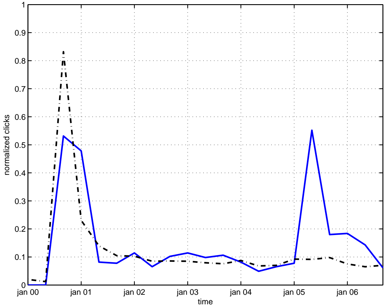
virasoro symmetry
