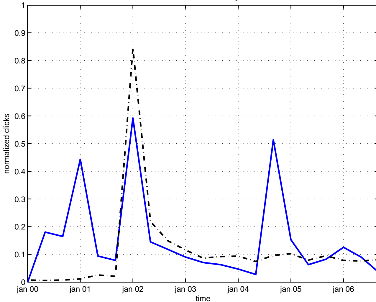
virasoro central charge
