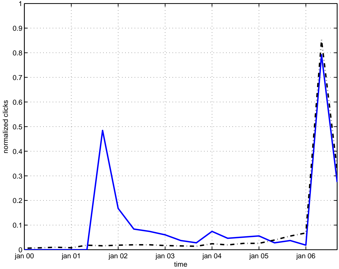
violation t-duality
